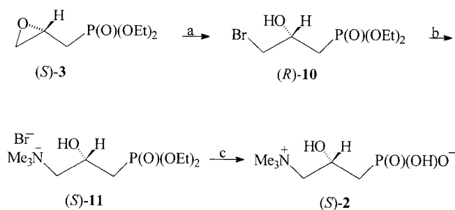
Scheme 3. Reagents and conditions: (a) MgBr 2 , diethyl ether; (b) 45% Me 3 N in ethanol/water; (c) 12 M HCl, H 2 O
