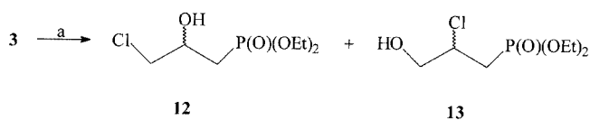
Scheme 4. Reagents and conditions: (a) 3.8 M HCl/EtOAc, 20 °C, 0.5 h
