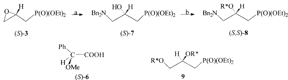
Scheme 2. Reagents and conditions: (a) Bn 2 NH (1.1 equiv.), 60 °C, 20 h; (b) 6 (1.5 equiv.), 1,3-dicyclohexylcarbodiimide (DCC) (1.5 equiv.), 4-(dimethylamino)pyridine (DMAP) (0.1 equiv.), CH 2 Cl 2
